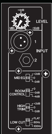
The rear panel of HS80M
